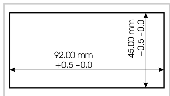
Figure 1-1 Panel Cut-out
