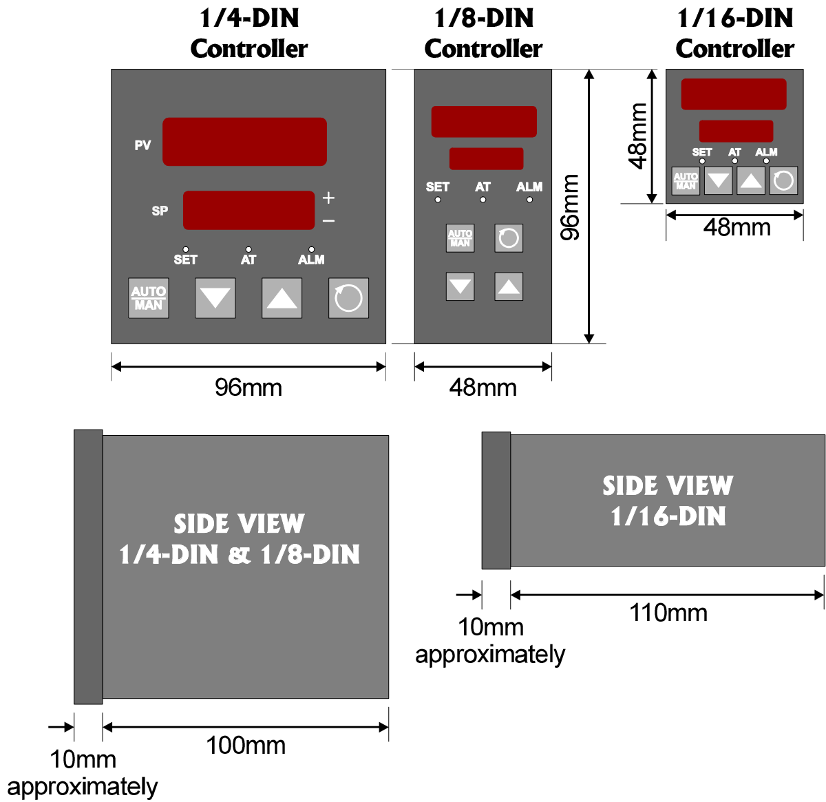
Figure 1-2 Principal Dimensions
