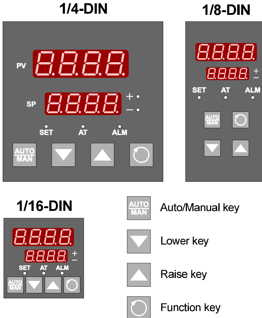
Figure 2-1 Front Panel Keys and Indicators
