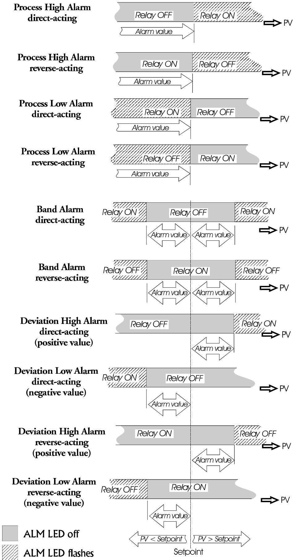
Figure 3-2 Alarm Operation
