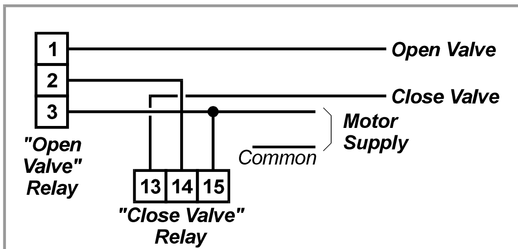
1/16-DIN Controller
