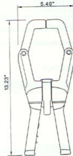
P3C Color: Red Cable: Size 3.27" Busbar Size: 4.8" x 2.13" or 4.0" x 2.5"
