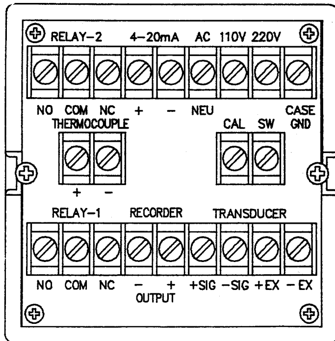
FIGURE B: Rear Terminal Assembly
