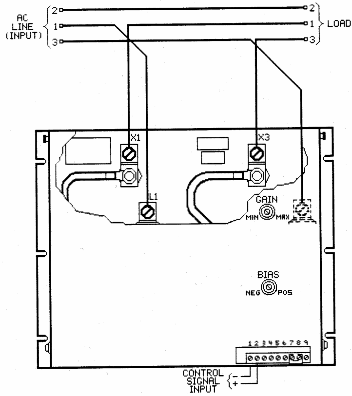
Figure 2-1. Typical 2Z Line and Load Connections
