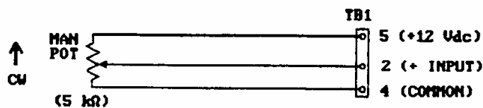
Figure 3-2. Remote control with a Potentiometer
