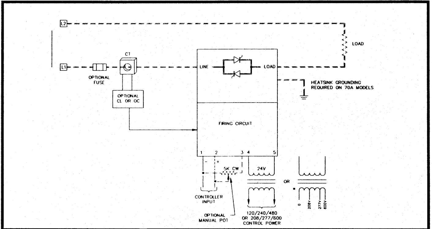
Typical Input/Output Connections for the 50P and the 100P
